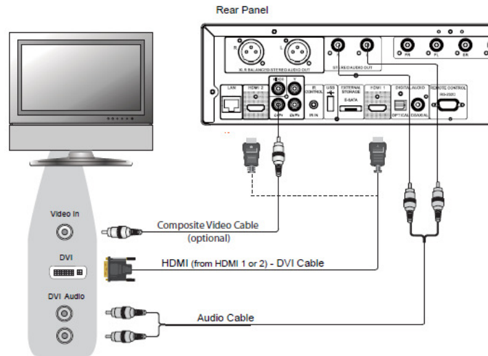
Method 3 – DVI Connection to TV
