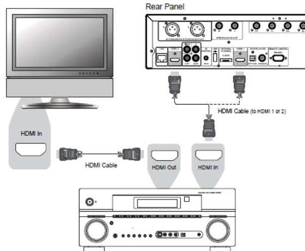
Method 5 – HDMI Connection to Receiver and TV
