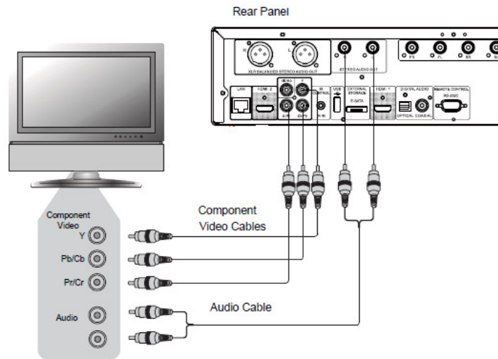
Method 4 – Component Video Connection to TV
