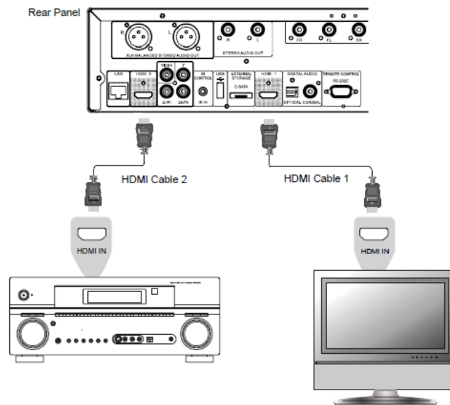
Method 9 – Dual HDMI Connection
