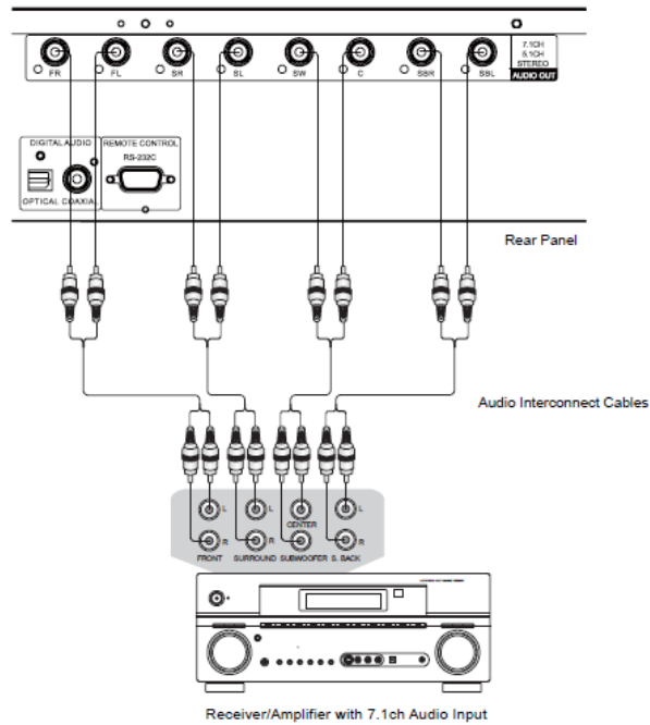
Method 6 – 7.1ch Analog Audio Connection
